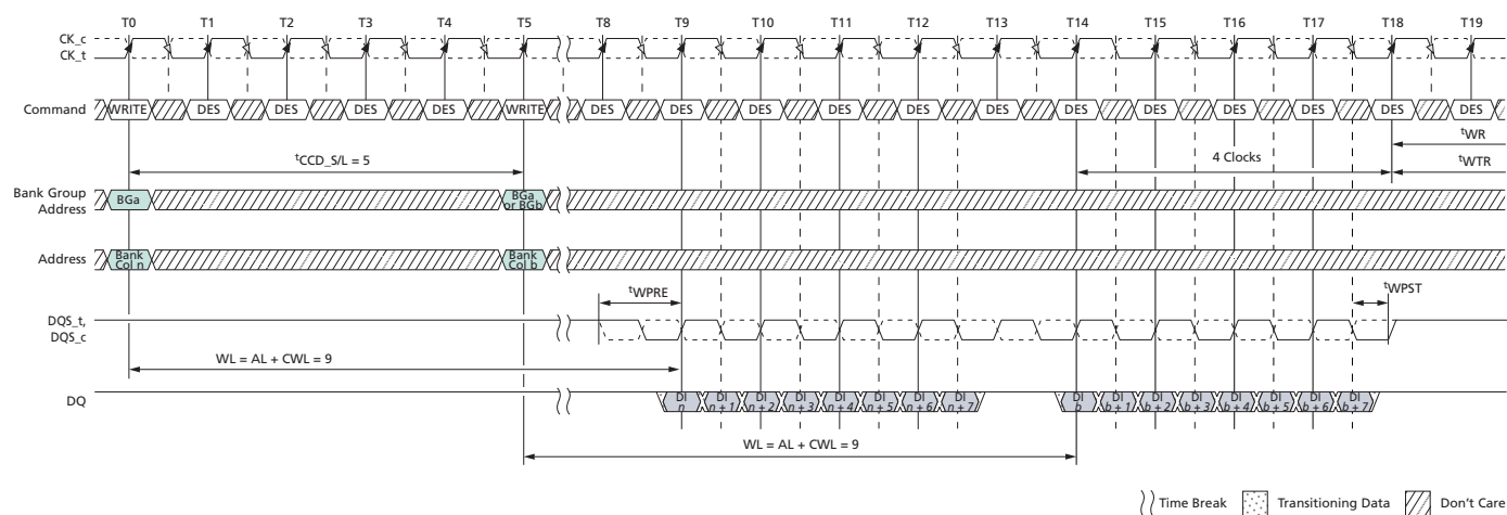
Figure 177: Nonconsecutive WRITE (BL8) with 1 st CK Preamble in Same or Different Bank Group
